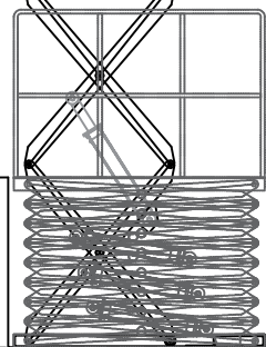
SIDE VIEW ALL ASSEMBLY WITHOUT SUPERSTRUCTURE
