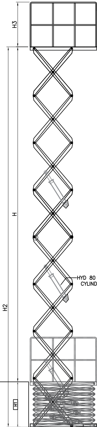
SIDE VIEW ALL ASSEMBLY WITHOUT SUPERSTRUCTURE
